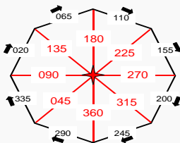
Example sector search Bearing to wpt. in red interim headings in black - use up to 3 NM from
